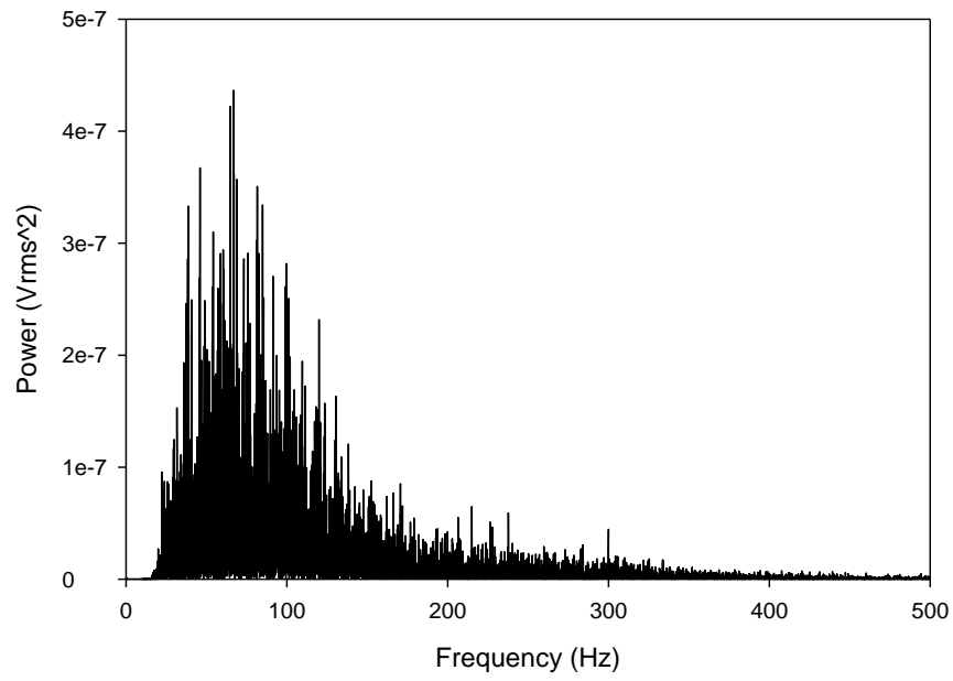
Figure 6. Frequency spectrum of raw sEMG data
