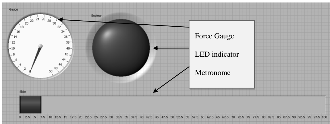
Figure 4. Custom program for control of isometric gripping trials
