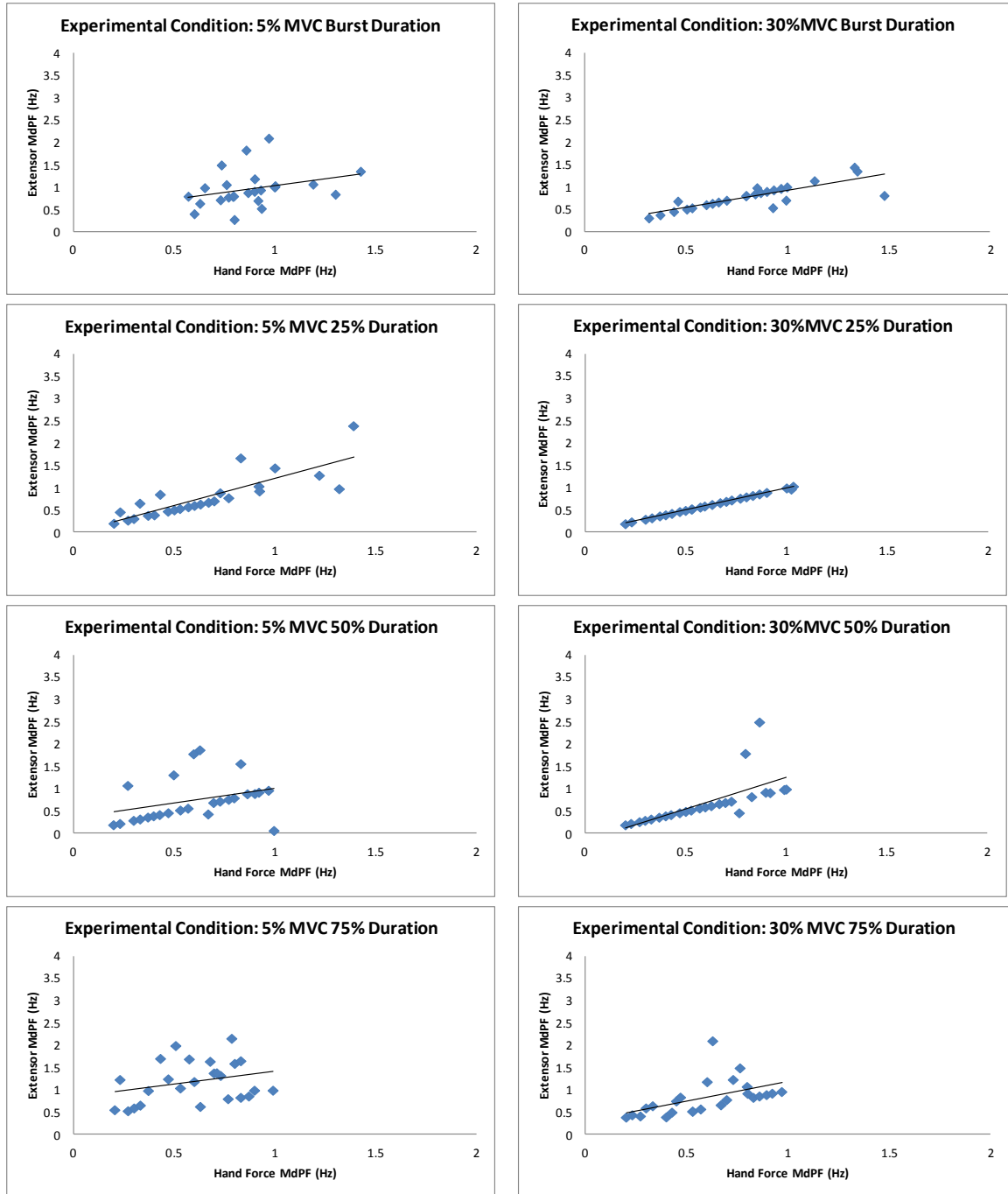
Figure 17. Scatter plots for MdPF_{HF} vs. MdPF_{EMG} (extensor muscles) for every combination of intensity (%MVC) and duration
